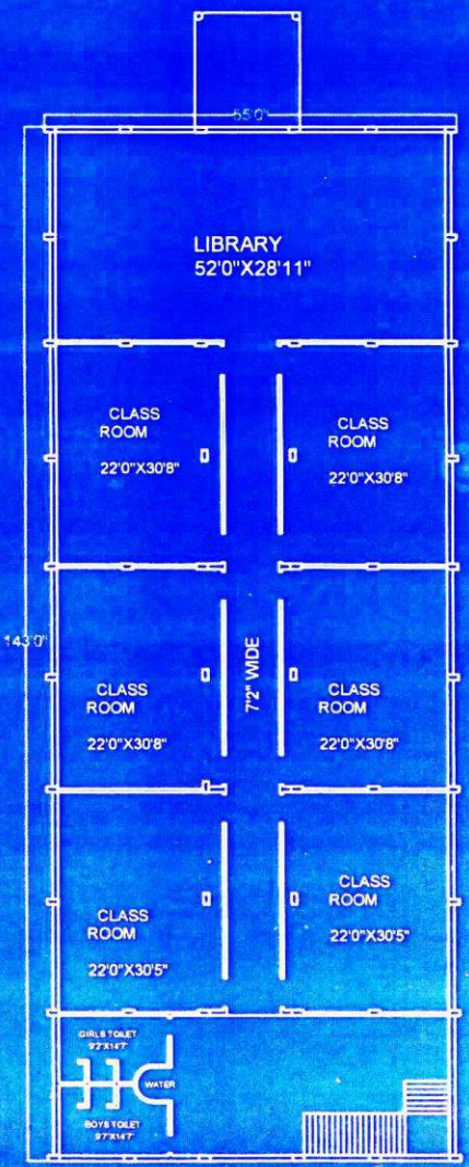
FIRST FLOOR PLAN-1
