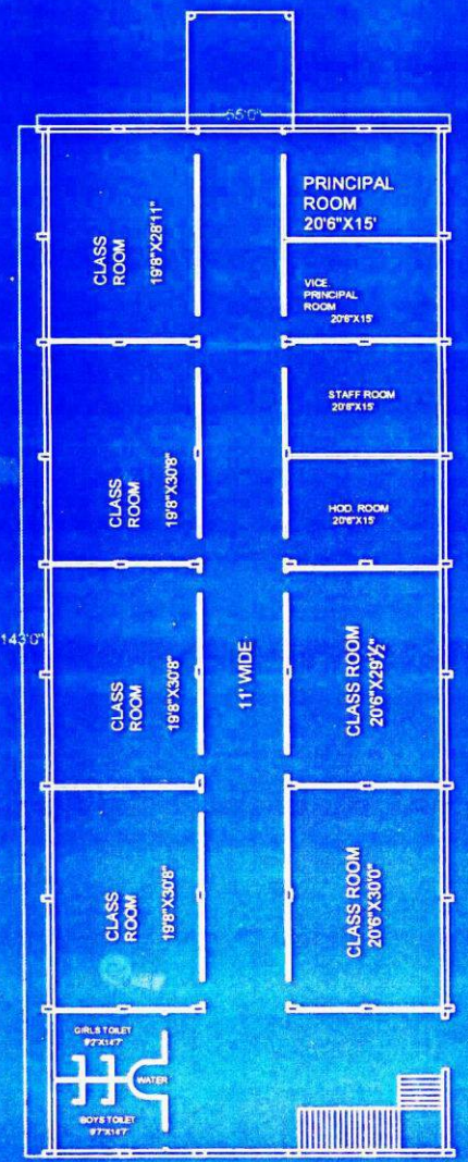
GROUND FLOOR PLAN-1
